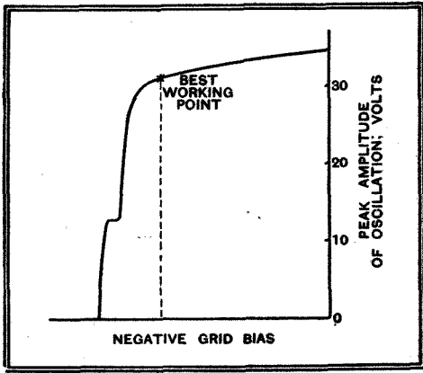
Fig. 4.—Graph showing correct operating point in relation to grid bias.
