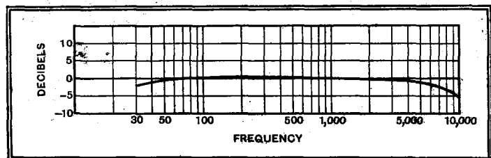
Overall characteristic curve of Trix model T.262 power amplifier, including the output transformer.
