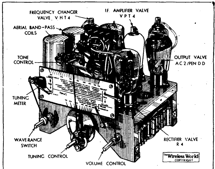
The "tell-tale" tuning panel is a special feature of the Lancastria set.
