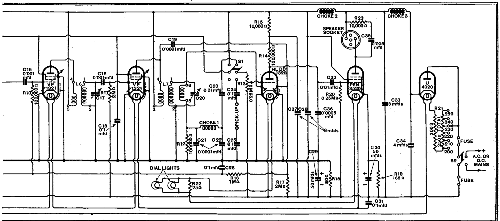
single-span tuning are retained. The valves all consume 0.2 ampere and their heaters are connected in series. The half-wave rectifier provides mains, and on a D.C. supply it protects the electrolytic condensers from damage.
