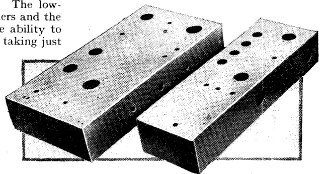
Metal chassis made by the London Radio Development Services, for the A.C. Single-Span receiver
