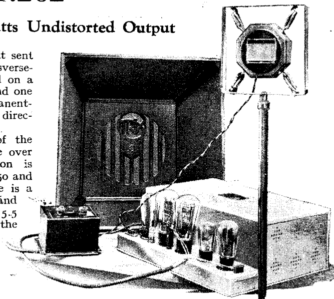
Trix public-address apparatus comprising model T.262 amplifier, microphone, and super-power P.M. loud speaker fitted in small directional baffle.
