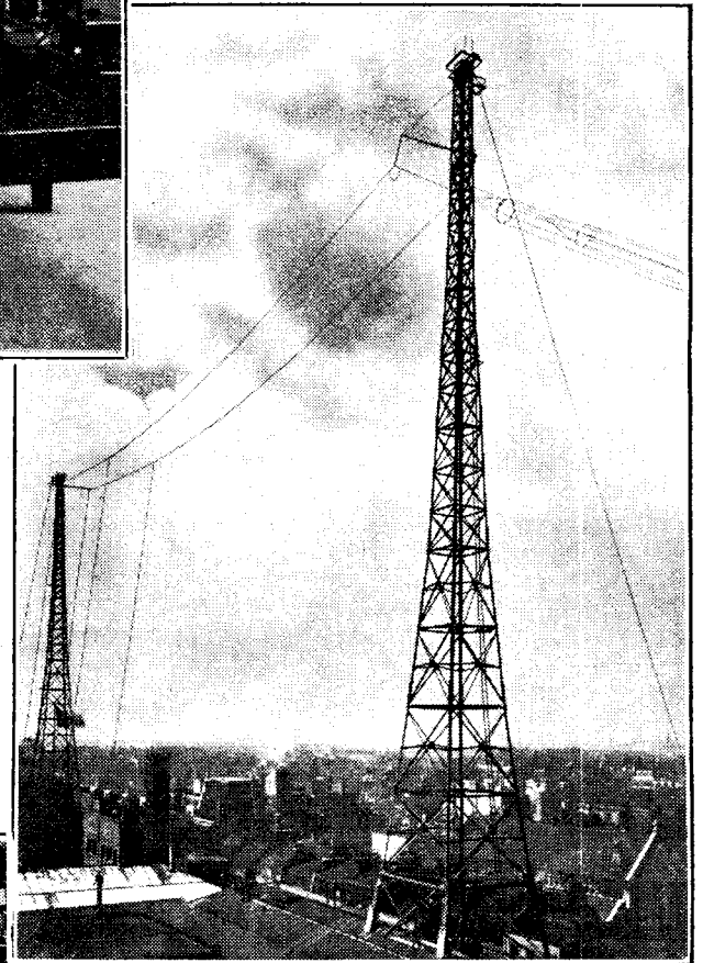
"2LO." The London masts on the roof of the Selfridge building in 1925. The transmitter had an aerial power of 2 kW.
