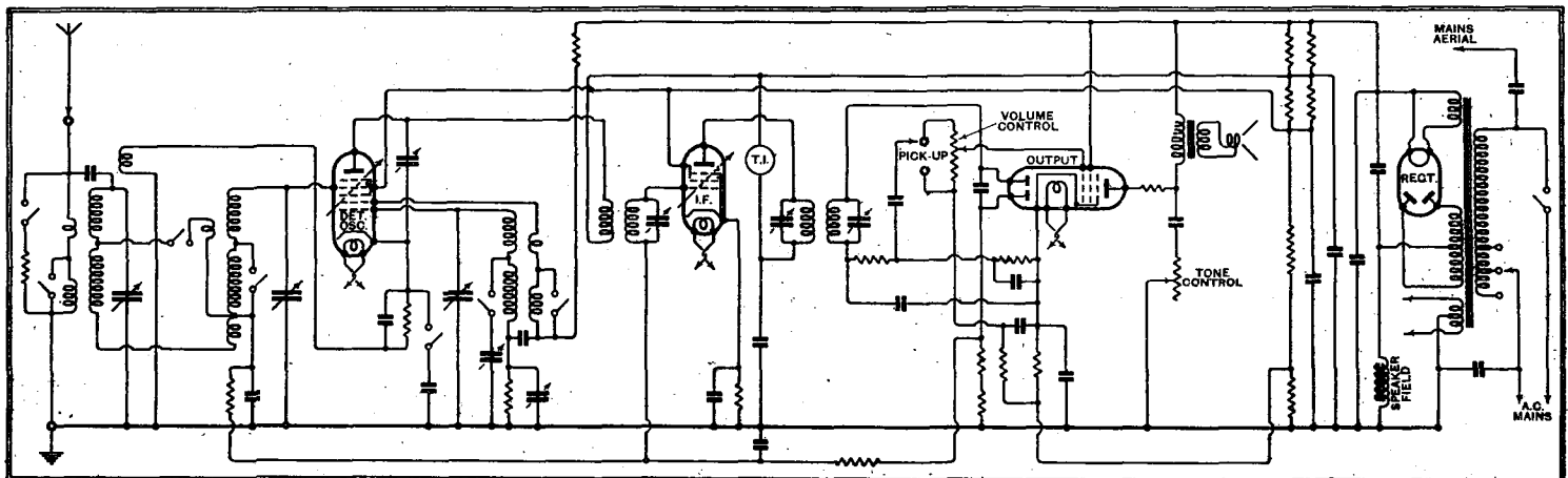
Ignoring the power rectifier and A.V.C. diode, there are five valve stages, but only three receiver valves.
