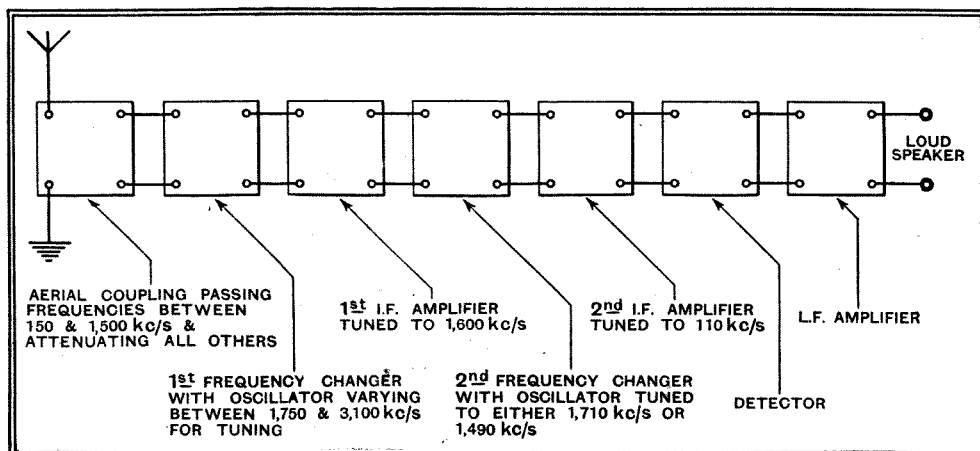
Fig. 1.—The general scheme of a single-span receiver embodying double-frequency-changing is illustrated here.
