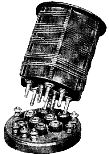
Eelex reversible Duplex dual-range short-wave coil.
