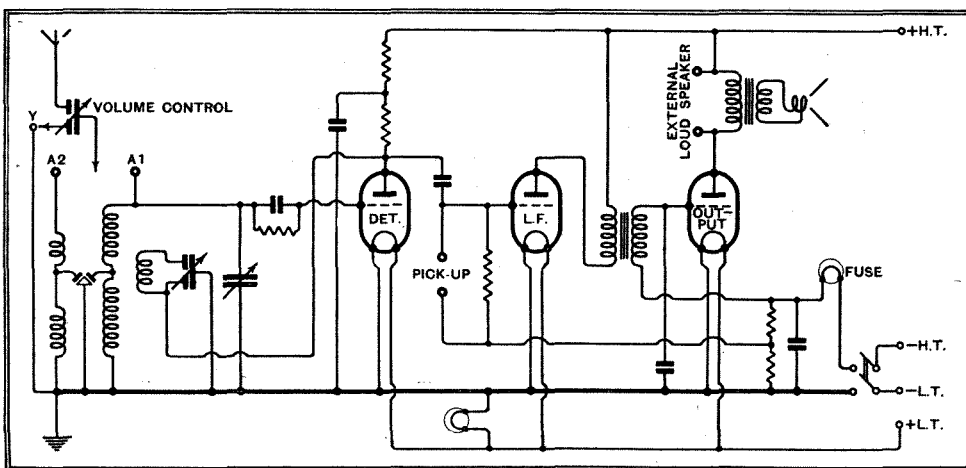
Complete circuit diagram. Automatic bias is provided and the aerial circuit may be modified to conform with the local conditions of reception.
