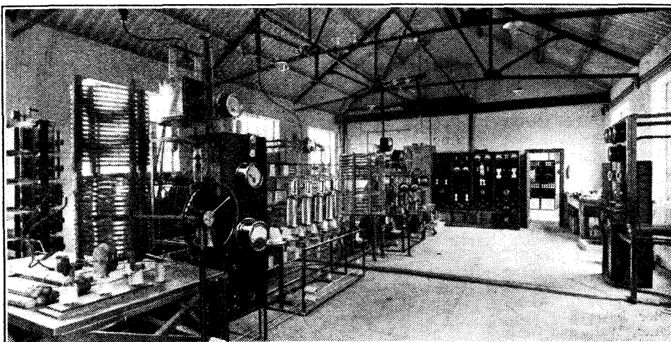
General view of the 5GB transmitter. The final stage of the power amplifier is in the centre background.
